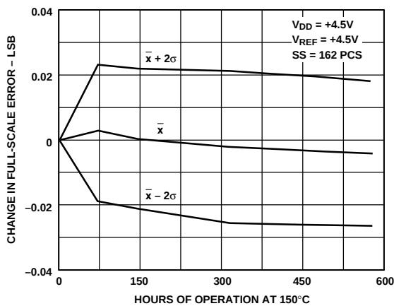
Figure 19. Full-Scale Error Accelerated by Burn-In
