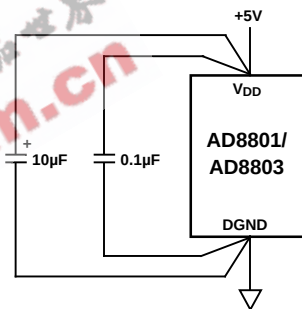
Figure 22. Recommended Supply Bypassing for the AD8801/AD8803
