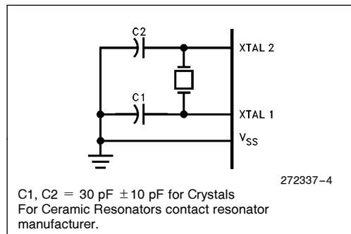
Figure 4. Oscillator Connections
