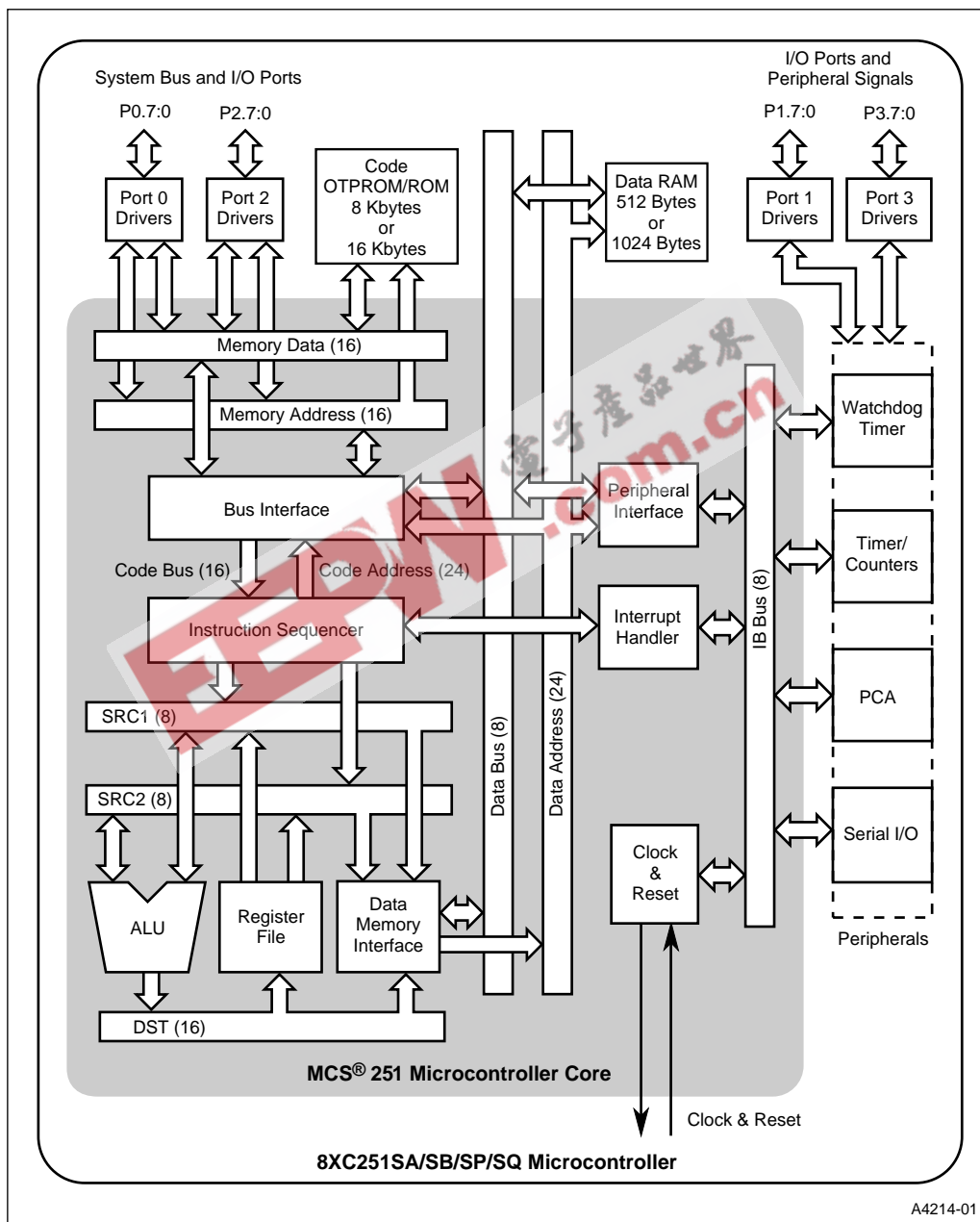
Figure 1. 8XC251SA/SB/SP/SQ Block Diagram
