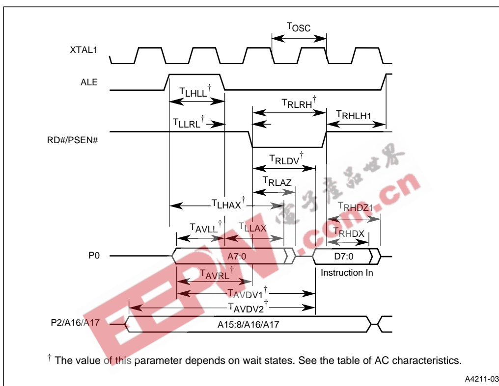
Figure 7. External Bus Cycle: Code Fetch (Nonpage Mode)
