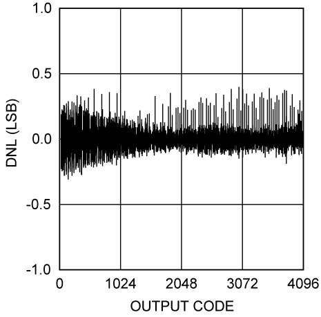
ADC121S101 DNL
