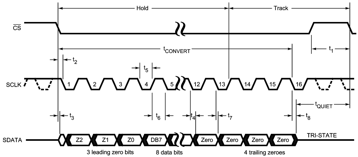
FIGURE 4. ADC081S101 Serial Interface Timing Diagram
