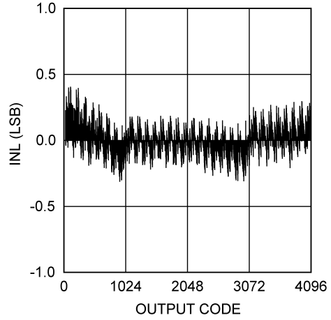
ADC121S101 INL
