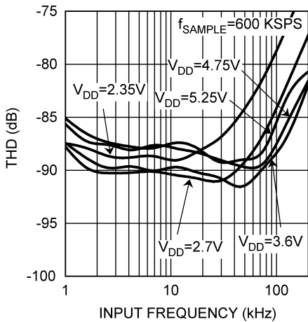
ADC121S101 THD vs. Input Frequency, 600 kSPS
