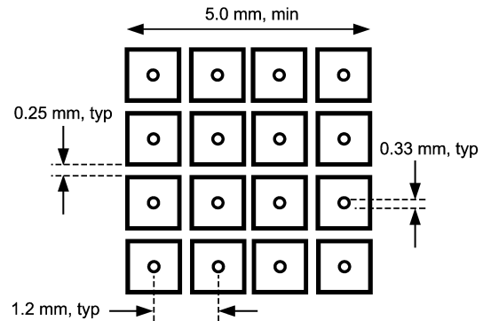
FIGURE 16. Recommended Package Land Pattern
