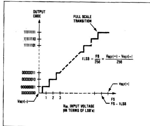
Figure 6. Transfer Function
