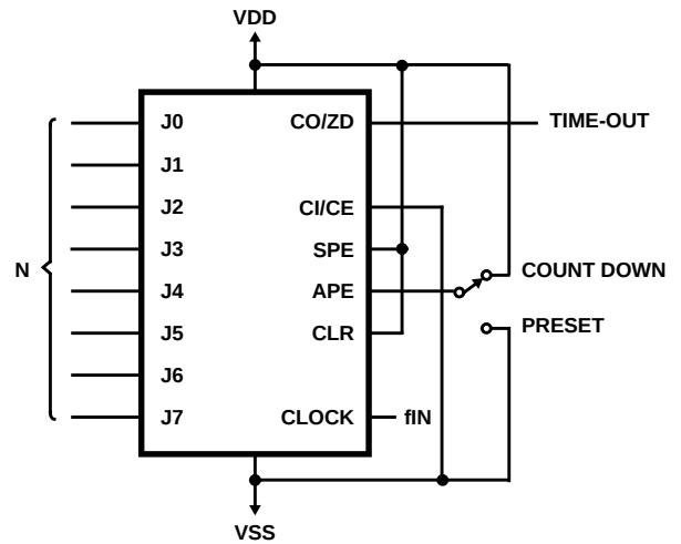
FIGURE 14. PROGRAMMABLE TIMER
