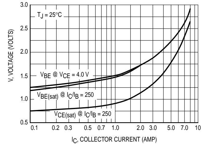
Figure 10. "On" Voltages
