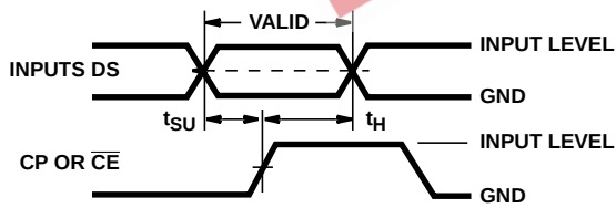
FIGURE 7. SERIAL-SHIFT MODE
