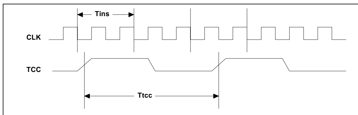
Fig. 4-17 TCC Input Timing (CLKS = "0") Timing Diagram
