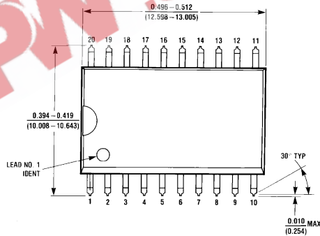
20-Lead Ceramic Dual-In-Line Package (J) Order Number DM54LS323J NS Package Number J20A
