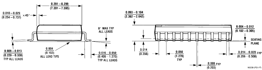
20-Lead Wide Small Outline Molded Package (M) Order Number DM74LS323WM NS Package Number M20B
