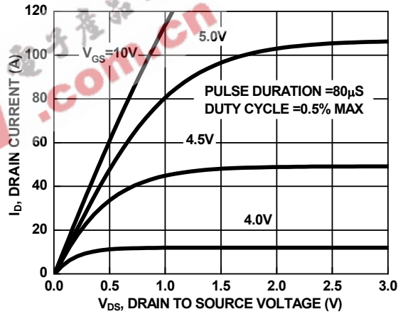
Figure 8. Saturation Characteristics
