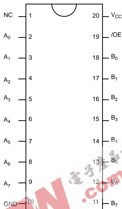
Figure 2. Pin Configuration
