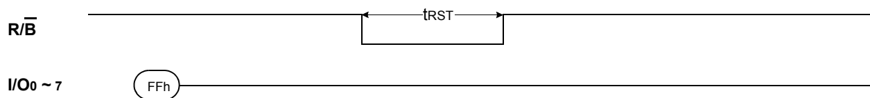
Figure 10. RESET Operation
