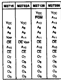
Figure 2. Pin Configurations
