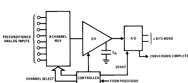
FIGURE 5. Random-Addressed, Multiplexed DAU
