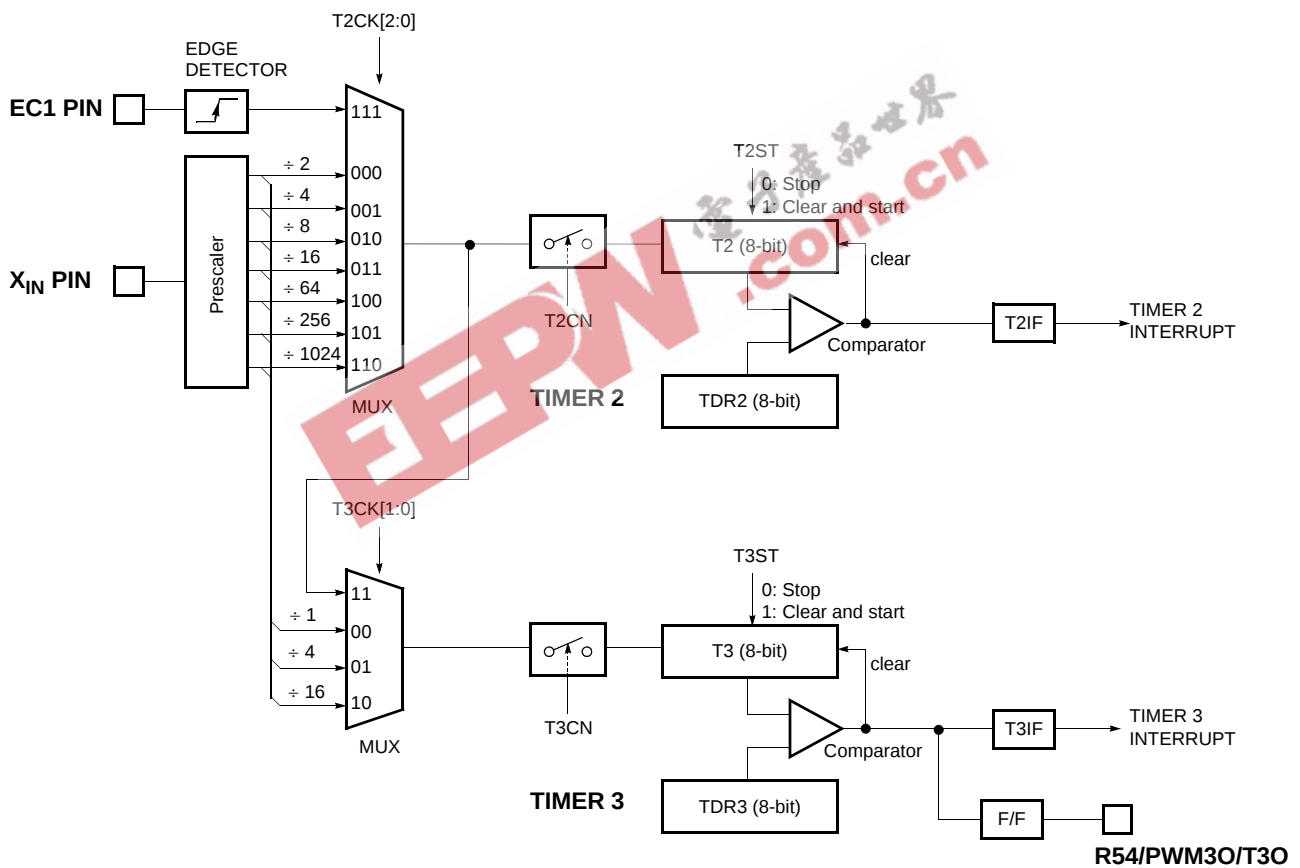
Figure 14-5 8-bit Timer/Counter 2, 3
