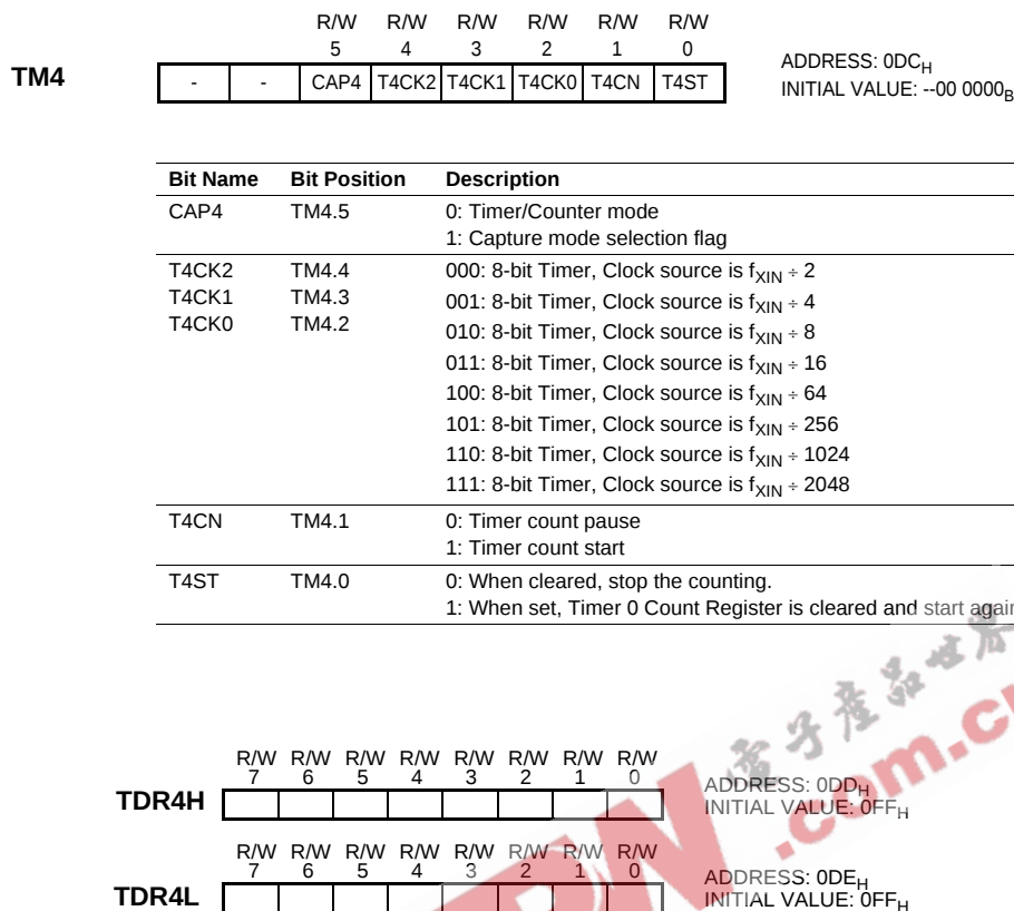
Figure 14-3 TM4 Register
