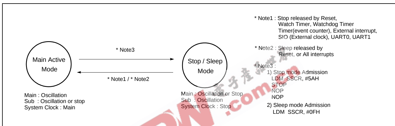
Figure 20-1 Operating Mode
