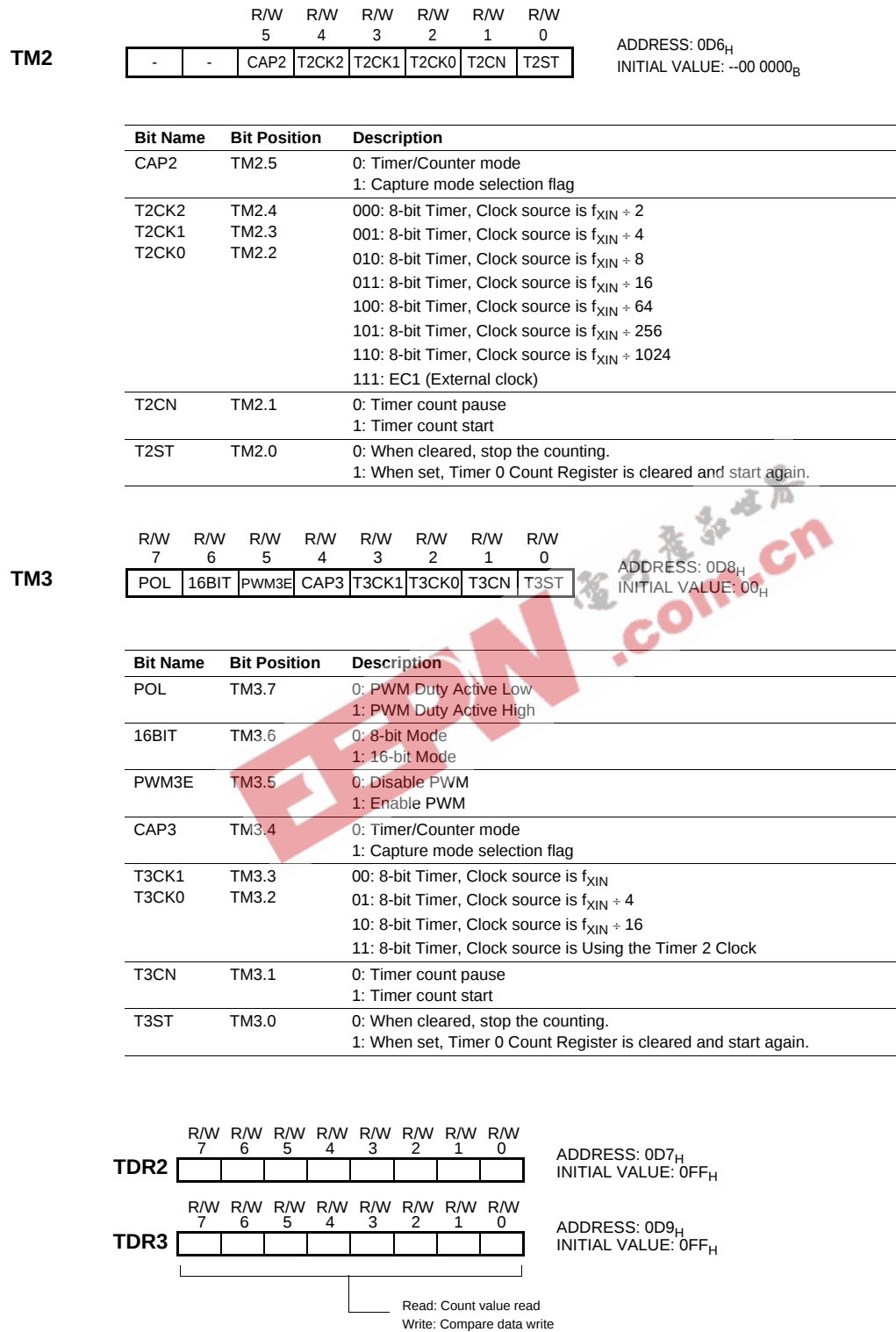
Figure 14-2 TM2, TM3 Registers
