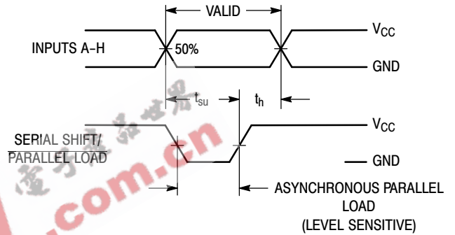
Figure 6. Parallel-Load Mode
