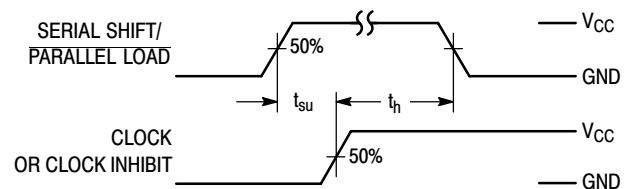
Figure 8. Serial-Shift Mode
