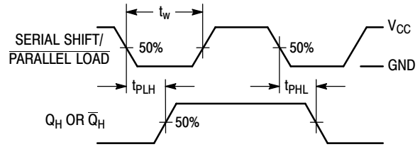
Figure 4. Parallel-Load Mode
