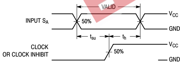
Figure 7. Serial-Shift Mode
