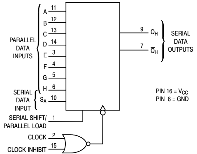
Figure 2. Logic Diagram
