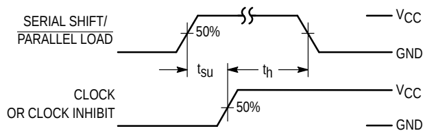
Figure 6. Serial-Shift Mode
