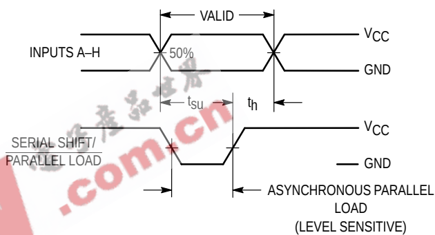
Figure 4. Parallel-Load Mode
