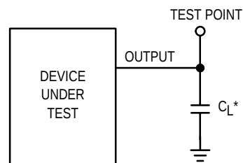
Figure 8. Test Circuit
