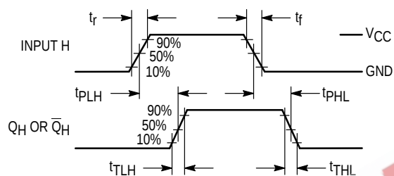
Figure 3. Parallel-Load Mode
