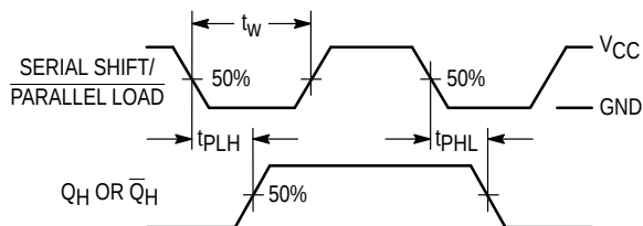
Figure 2. Parallel-Load Mode
