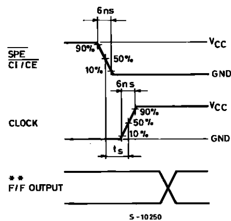
WAVEFORM 5
