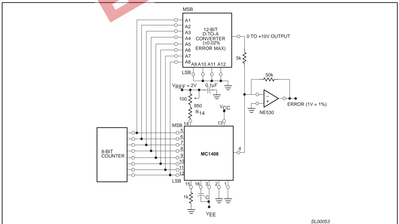
Figure 6. Relative Accuracy
