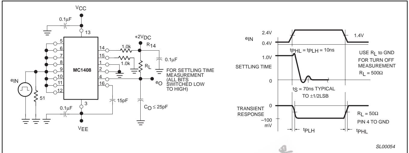
Figure 7. Transient Response and Settling Time
