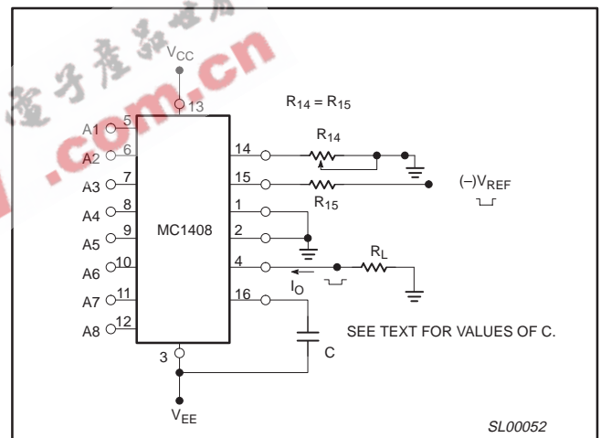
Figure 5. Negative V_{REF}
