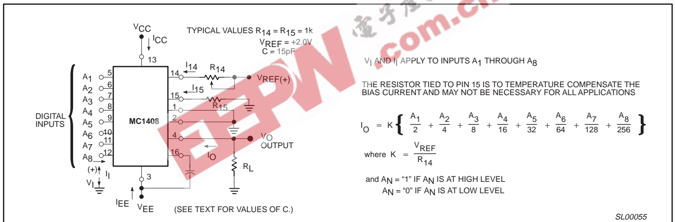
Figure 8. Notation Definitions
