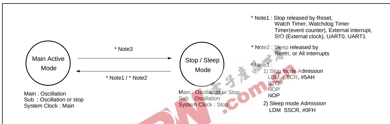
Figure 20-1 Operating Mode
