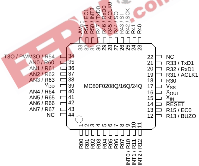
44MQFP (Top View)
