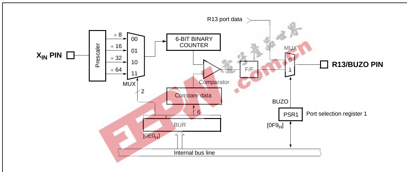
Figure 18-1 Block Diagram of Buzzer Driver
