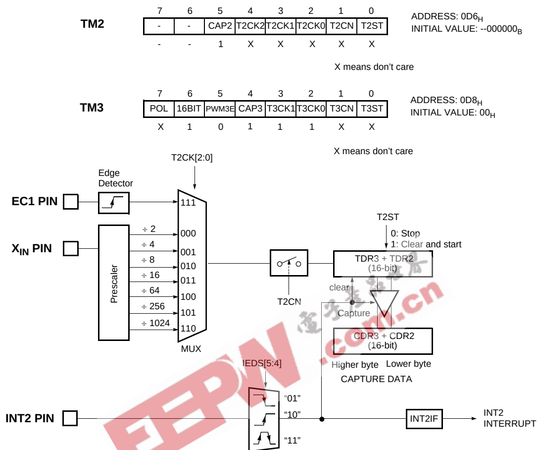
Figure 14-18 16-bit Capture Mode of Timer 2, 3
