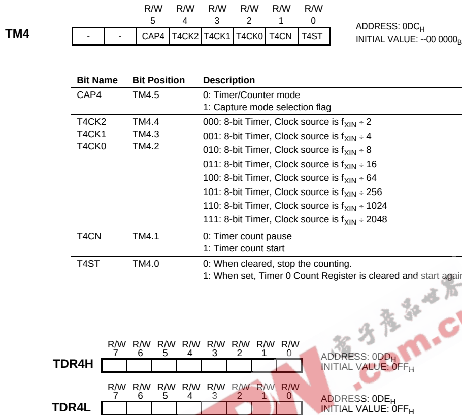
Figure 14-3 TM4 Register
