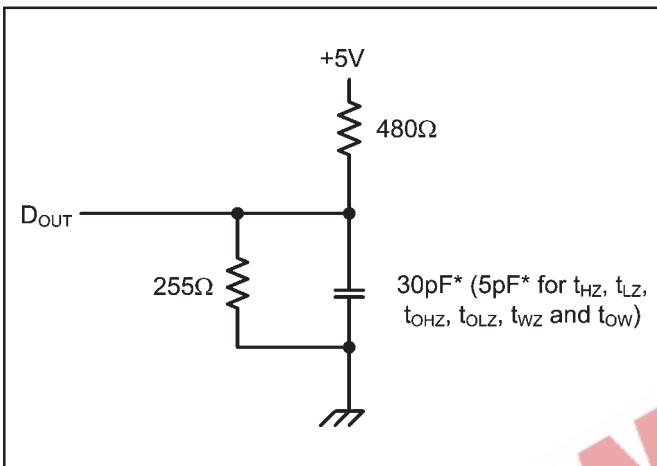
Figure 1. Output Load
