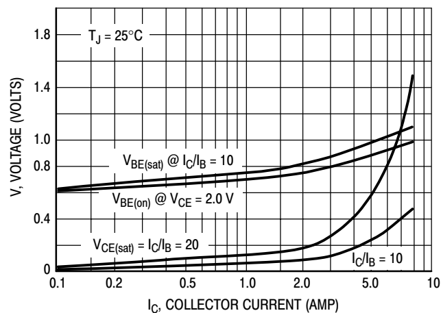
Figure 9. "On" Voltage
