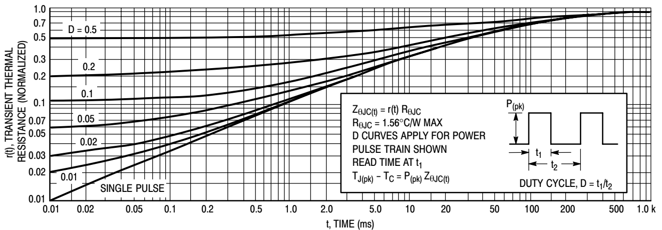
Figure 2. Thermal Response
