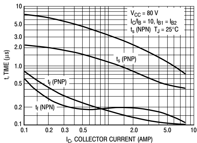
Figure 11. Turn-Off Times
