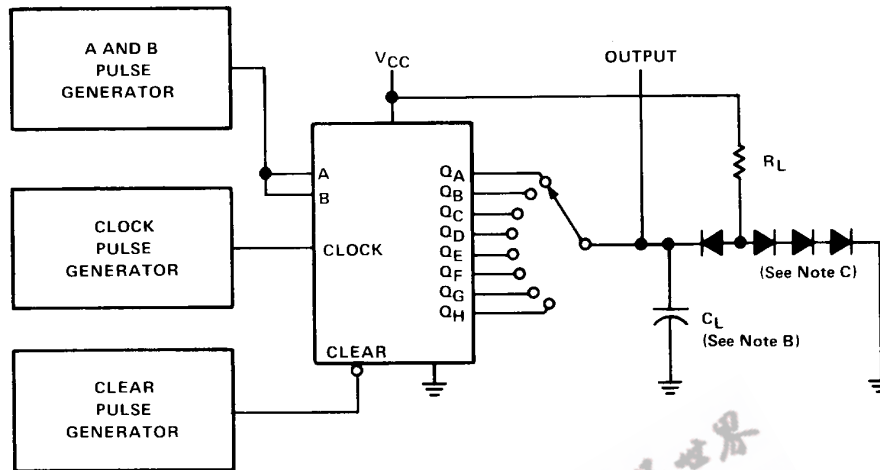
TEST CIRCUIT
