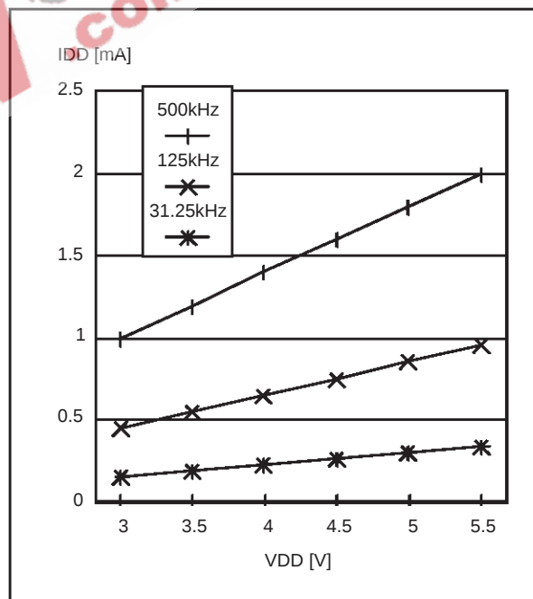
Figure 70. Typical I_{DD} in SLOW vs. f_{CPU}
