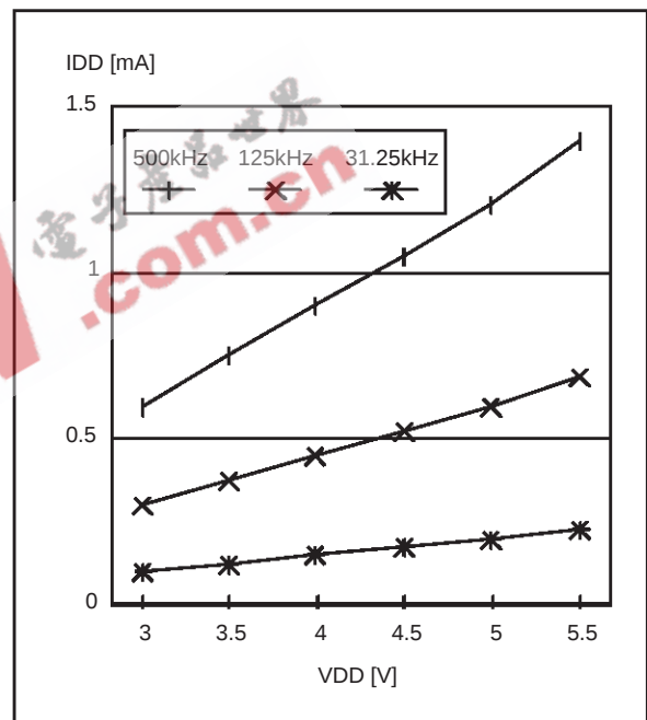
Figure 72. Typical I_{DD} in SLOW-WAIT vs. f_{CPU}
