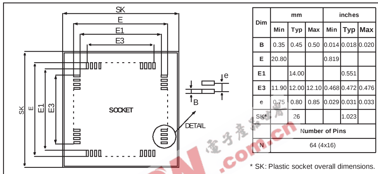
Figure 97. TQFP64 Device And Emulator Probe Compatible Footprint
