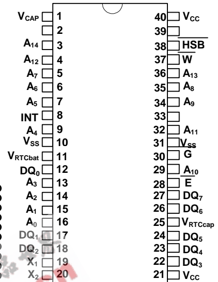
40 Pin PDIP
