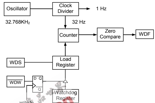
Figure 7. Watchdog Timer Block Diagram
