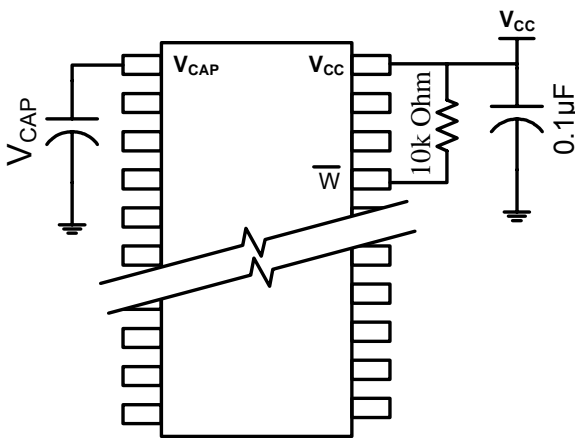
Figure 5: AutoStore™ Mode
