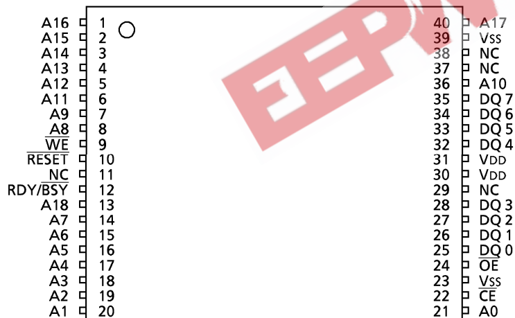
TC58FVT004FT / B004FT (TSOP Type - I)
