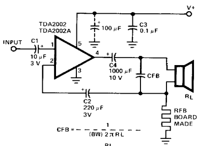
LOW COST APPLICATION CIRCUIT
