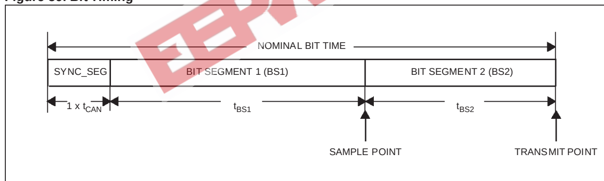
Figure 59. Bit Timing
