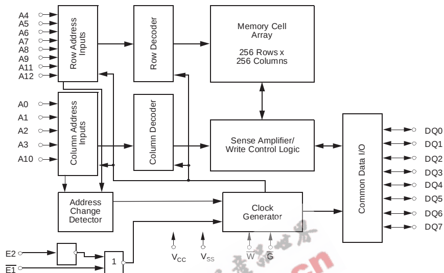
Block Diagram
