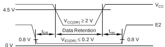
Data Retention Mode E2-Controlled
