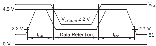
Data Retention Mode \overline{E1} -Controlled
