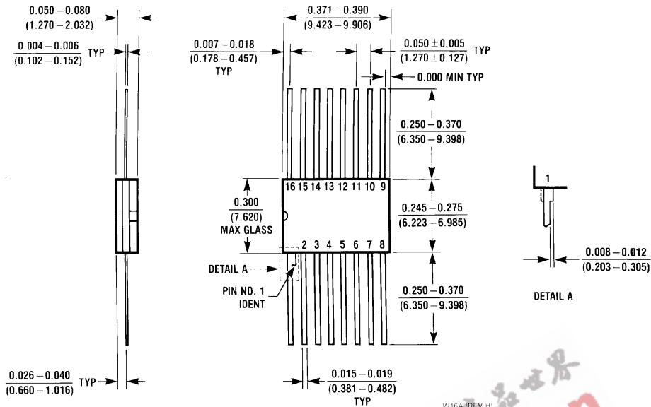
16-Lead Ceramic Flat Package (W) Order Number 9314FMOB NS Package Number W16A
