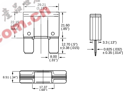
Reference Dimensions
