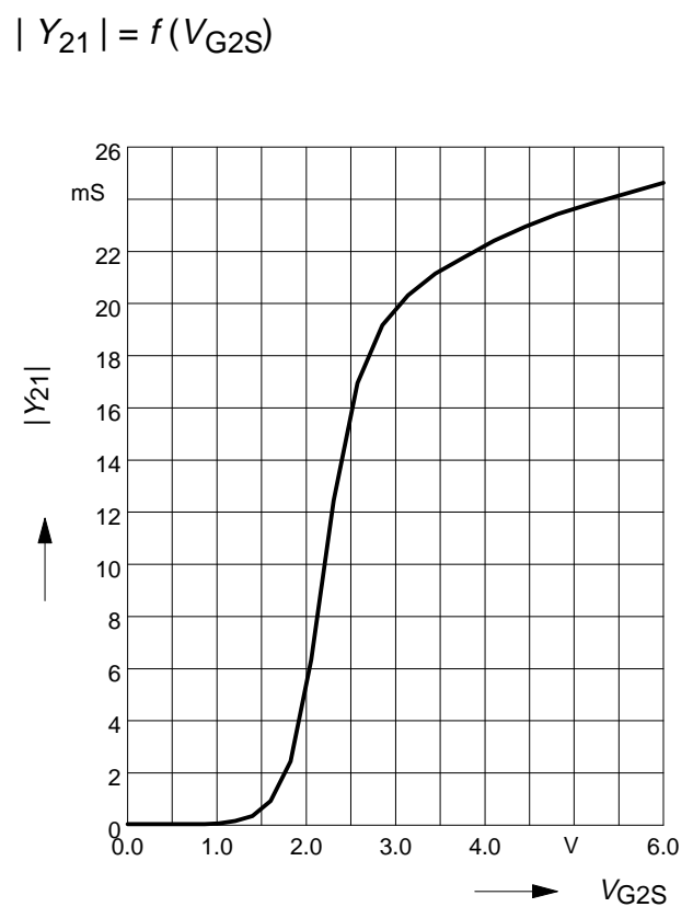
Forward transfer admittance |Y_{21}| = f(V_{G2S})
