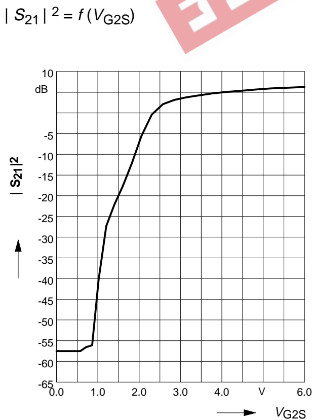
Insertion power gain |S_{21}|^2 = f(V_{G2S})
