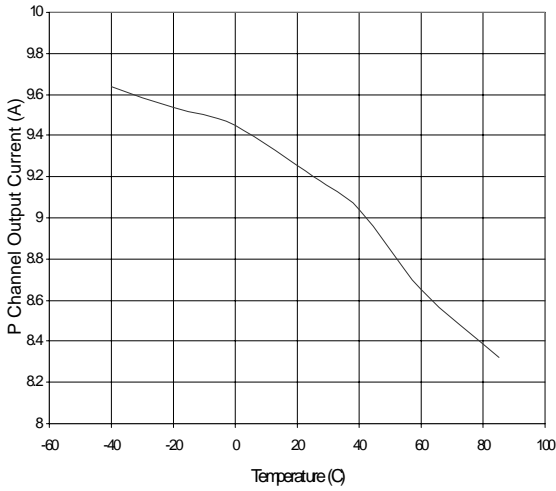
Fig. 21 P Channel Output Current vs. Temperature Vcc=18V/CL=10rF
