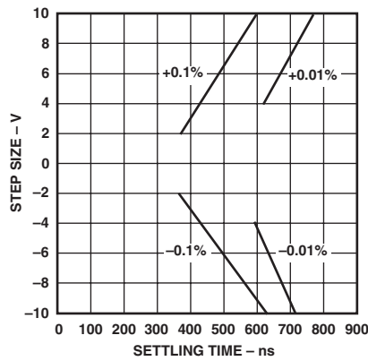
TPC 20. Settling Time vs. Step Size
