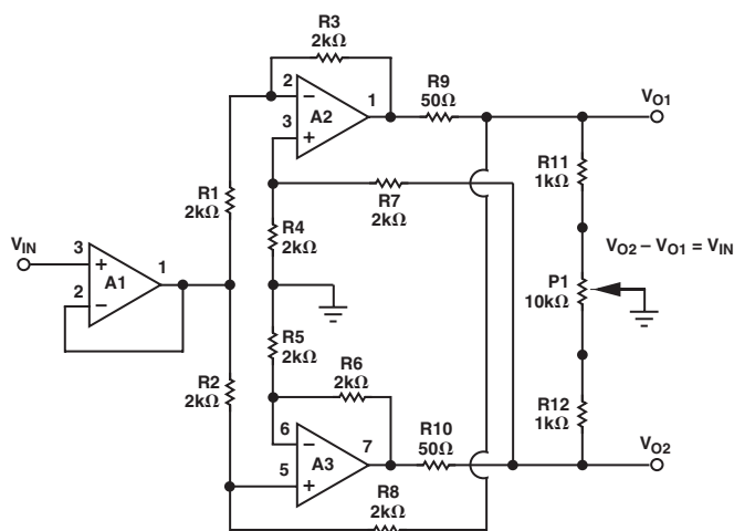
A1 = 1/2OP285 A2, A3 = 1/2 OP285 GAIN = SET R2, R4, R5 = R1 AND R, R7, R8 = R2
