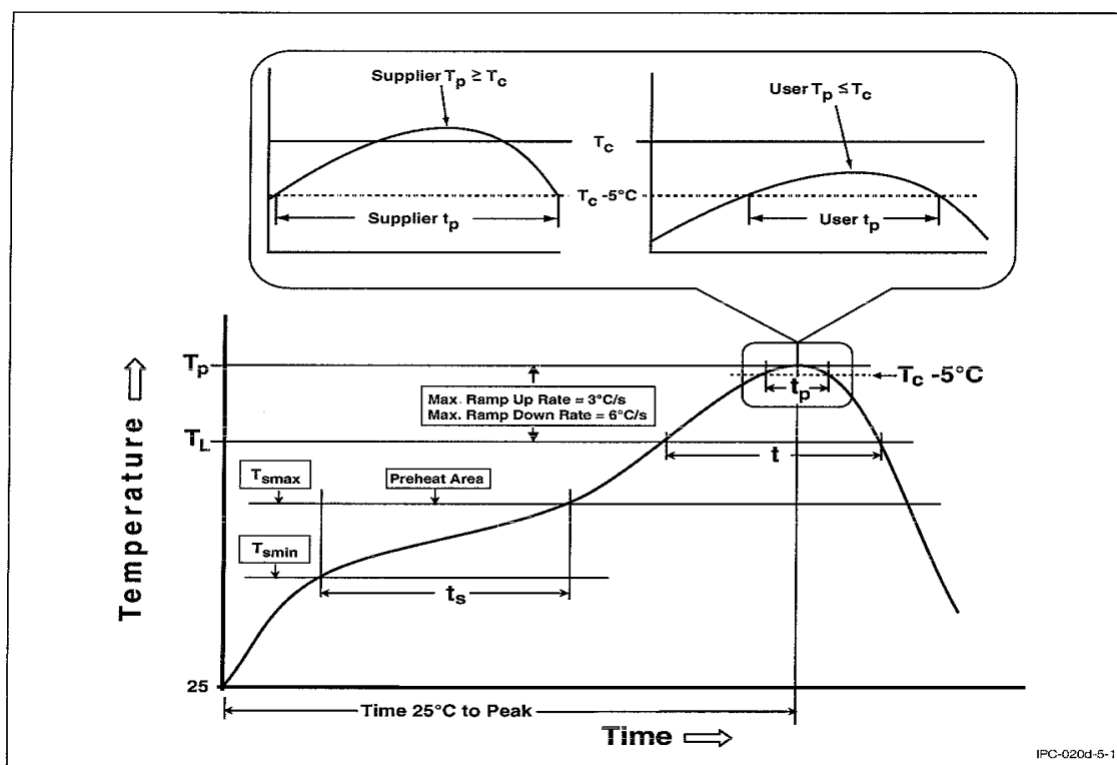
Recommended Reflow Profile
