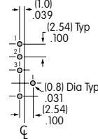
V Terminals
