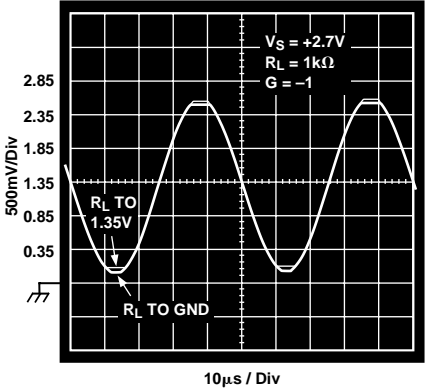
Figure 35. Output Swing
