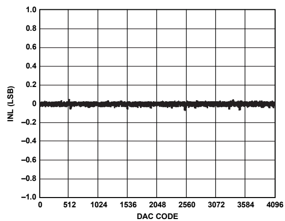
Figure 8. AD5025 INL
