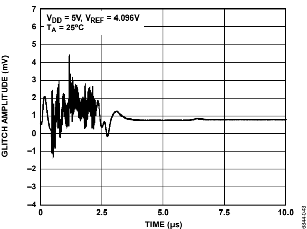
Figure 26. Analog Crosstalk
