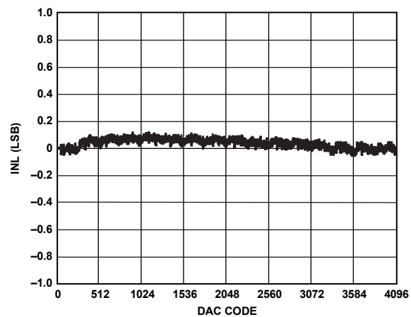
Figure 7. AD5045 INL
