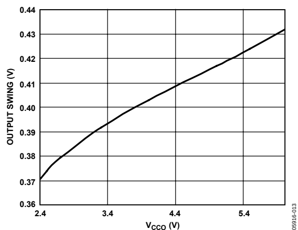
Figure 14. LVDS Output Swing vs. V_{CCO} (V)
