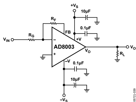
Figure 39. Inverting Gain
