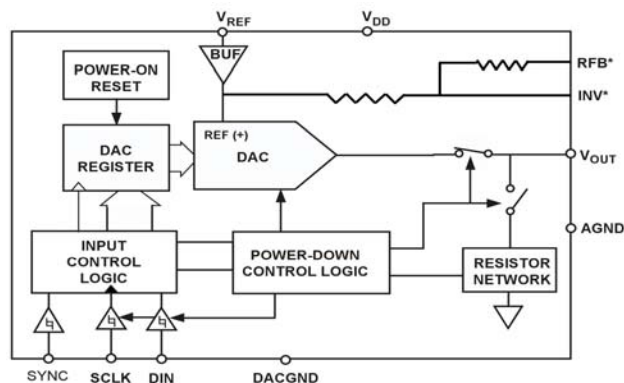
AD5063. 10 Ld MSOP.
