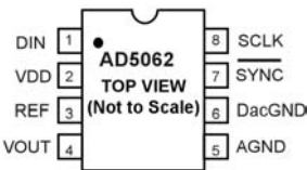
Figure 2. AD5062 8ld Sot23
