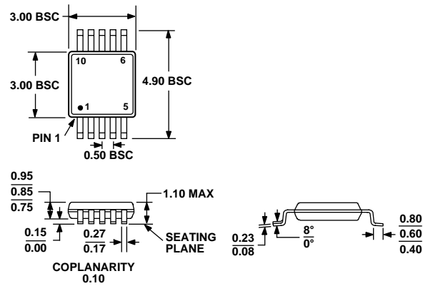
Figure 51. 10-Lead Mini Small Outline Package [MSOP] (RM-10)
