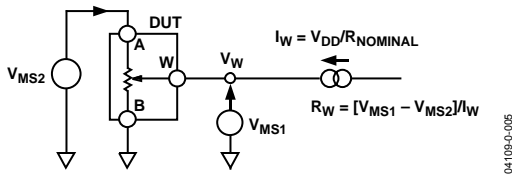
Figure 30. Test Circuit for Resistor Position Nonlinearity Error (Rheostat Operation; R-INL, R-DNL)
