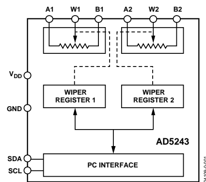
Figure 1. AD5243
