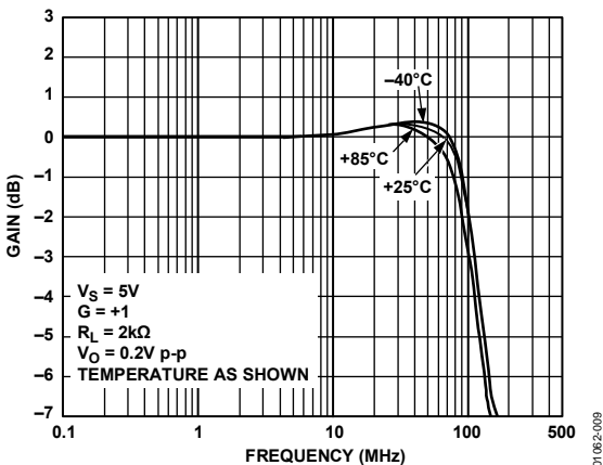
Figure 9. AD8051/AD8052 Gain vs. Frequency vs. Temperature
