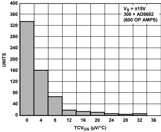
Figure 21. AD8682 TCV 0s Distribution SOIC_N Package
