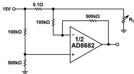
Figure 32. High-Side Signal Conditioning
