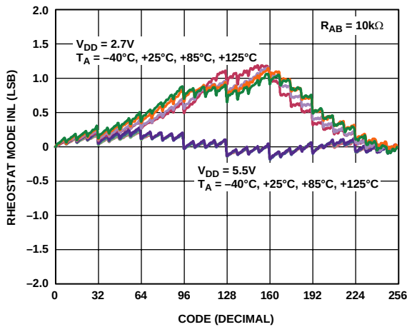
Figure 9. R-INL vs. Code vs. Temperature
