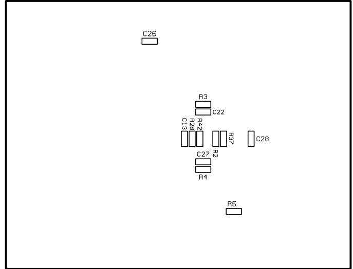
Figure 18. Assembly Bottom
